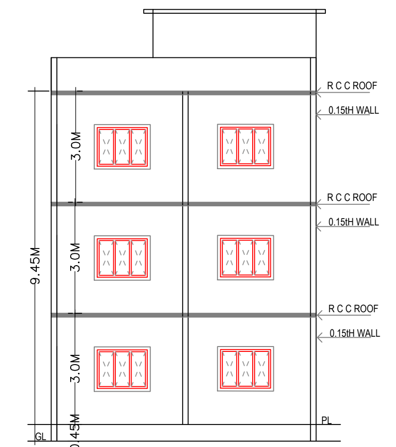
SECTION @ X-X
